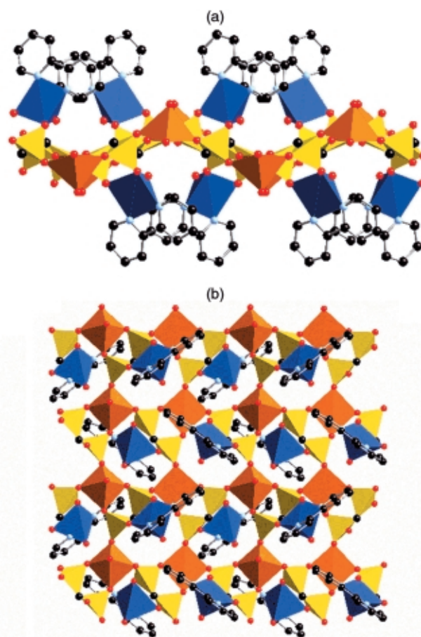
Fig. 1 (a) A view of the structure of [ \{\text{Cu}(2,2'\text{-bpy})(\text{H}_2\text{O})\}(\text{VO})(\text{O}_3\text{PCH}_2\text{PO}_3) ] ( 1 ), parallel to the oxide plane. (b) A polyhedral representation of the layer structure of 1 . Selected bond lengths (Å): Cu– \text{O}_{\text{aqua}} , 2.216(3); Cu– \text{O}_{\text{phosphonate}} , 1.933(2), 1.954(3); Cu–N, 2.033(3), 2.216(3); V– \text{O}_t , 1.593(3); V– \text{O}_{\text{phosphonate}} , 1.987(5), ave. of 4 V–O bonds. Abbreviations: \text{O}_t = terminal oxo-groups.
