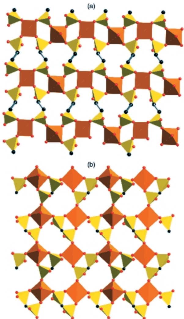
Fig. 2 Polyhedral representations of the (a) \{(VO)(O_3PCH_2PO_3)\}^{2-} and (b) \{(VO)(O_3PCH_2CH_2PO_3)\}^{2-} networks of 1 and 2 , respectively.
