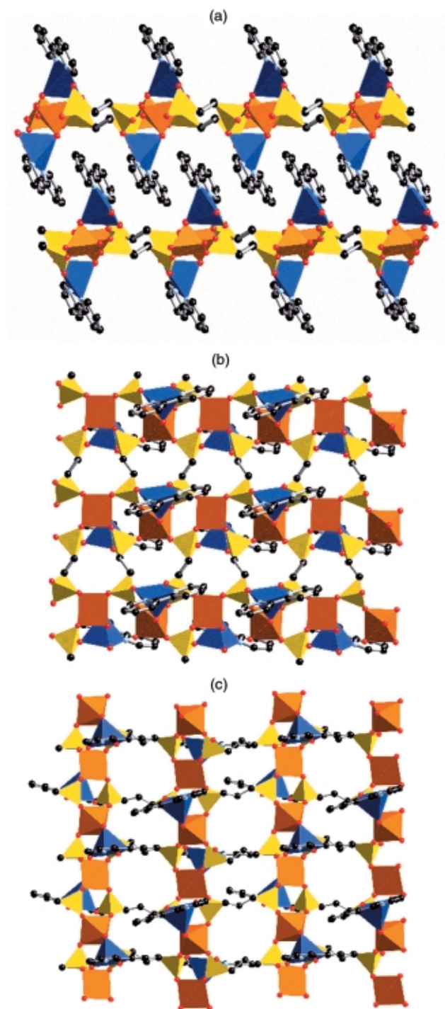
Fig. 3 (a) A view of the structure of [Cu(2,2'\text{-bpy})(VO)(O_3PCH_2CH_2PO_3)] ( 2 ), parallel to the oxide plane. (b) A polyhedral representation of the layer structure of 2 , showing the \{Cu(2,2'\text{-bpy})(VO)(O_3PR)_2\} chains, linked through ethylene bridges into a covalent network. Selected bond lengths (Å): Cu–O b (V), 2.394(2); Cu–O phosphonate , 1.919(2), 1.942(2); Cu–N, 2.006(2), 2.030(2); V–O b (Cu), 1.611(2); V–O phosphonate , 1.962(4), ave of 4 V–O bonds. (c) A view of the structure of [Cu(2,2'\text{-bpy})(VO)(O_3PCH_2CH_2CH_2PO_3)]\cdot H_2O ( 3 ), normal to the oxide plane. Selected bond lengths (Å), averages: Cu–O b (V), 2.387(7); Cu–O phosphonate , 1.920(8); Cu–N, 2.000(9); V–O b (Cu), 1.605(7); V–O phosphonate , 1.973(8). Abbreviations: O b = bridging oxo-groups.
